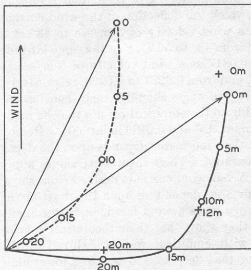
Fig. 122. Wind current in shallow water assuming a constant eddy viscosity ( dashed curve ) or an eddy viscosity which decreases towards the bottom ( full-drawn curve ). Observed currents indicated by crosses.
