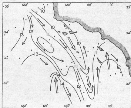
Fig. 126. Tonguelike distribution of temperature at a depth of 50 m off southern California in May, 1937. Solid arrows indicate direction of flow according to the geopotential topography of the sea surface; open arrows show the axes of the tongues.
