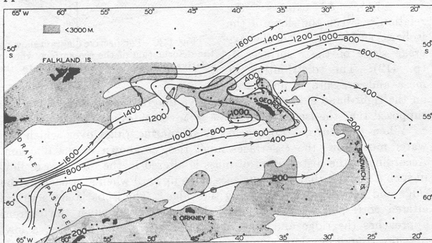
Fig. 117. Topography of the surface \sigma_t = 27.7 in the area from the Drake Passage to the east of South Sandwich Islands.
