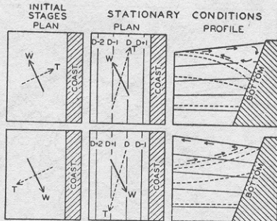
FIG. 124. Schematic representation of effect of wind towards producing currents parallel to a coast in the Northern Hemisphere and vertical circulation. W shows wind direction, and T , direction of transport. Contours of sea surface shown by lines marked D , D + 1 . . . . Top figures show sinking near the coast; bottom figures show upwelling.
