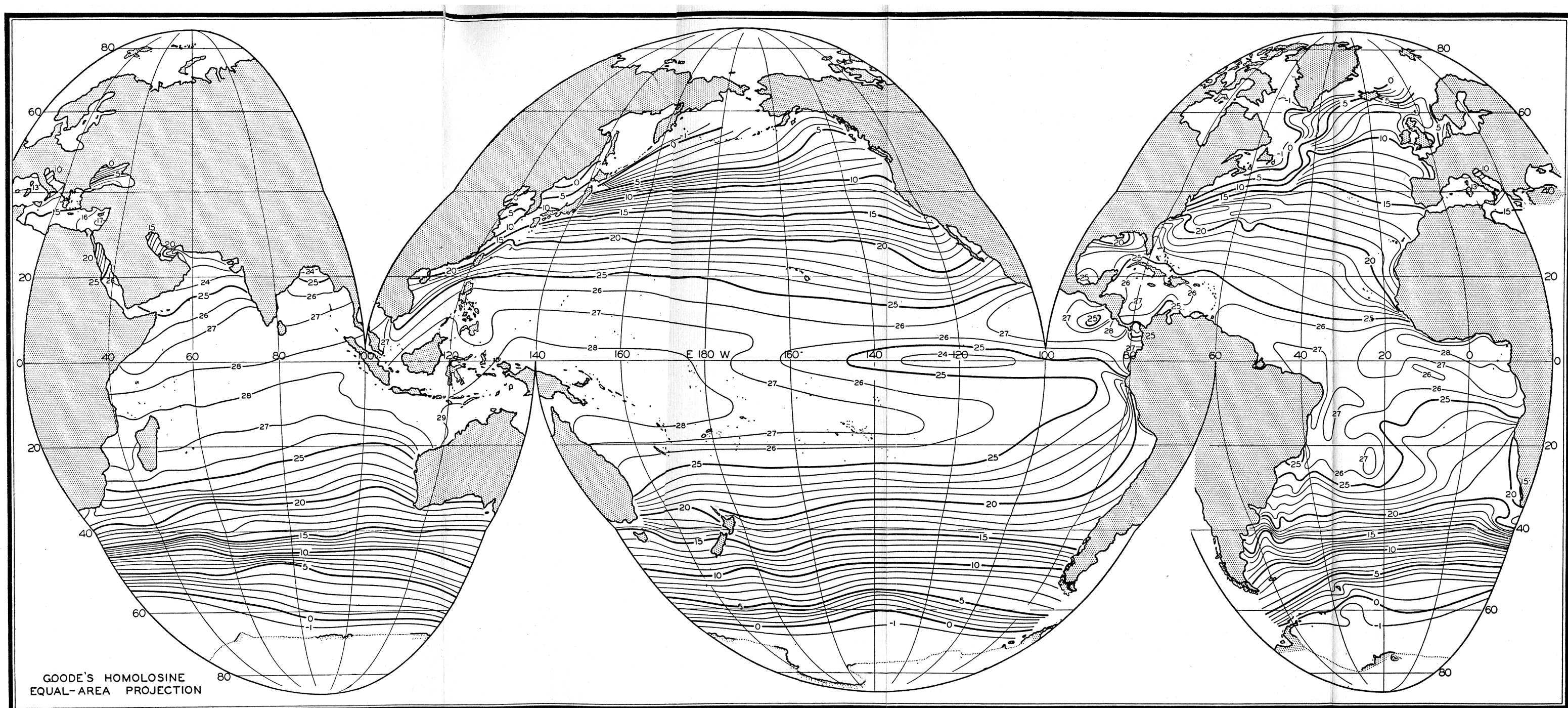
Chart II. Surface temperature of the oceans in February.
